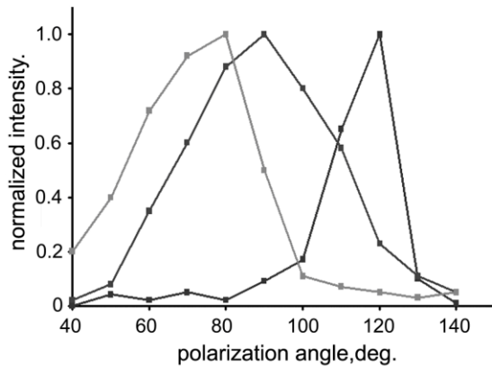
Fig. (4) Integral intensity of “hot spots” luminescence with various polarization of laser pulse
