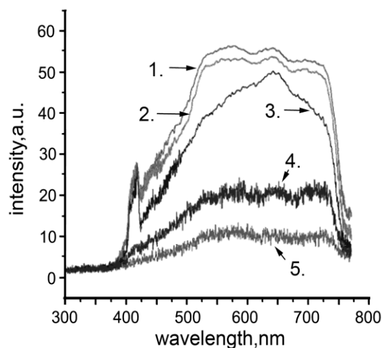
Fig. (3) Luminescence spectra from various pixels of the Au/TiO 2 mesoporous film in two-photon microscopy experiment
