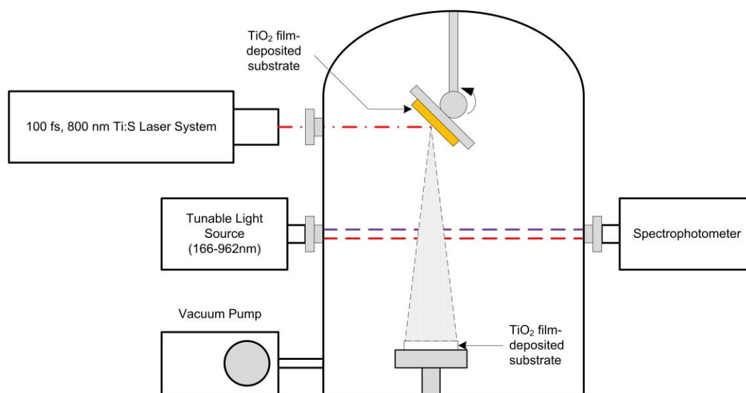
Fig. (1) Experimental setup used in this work
