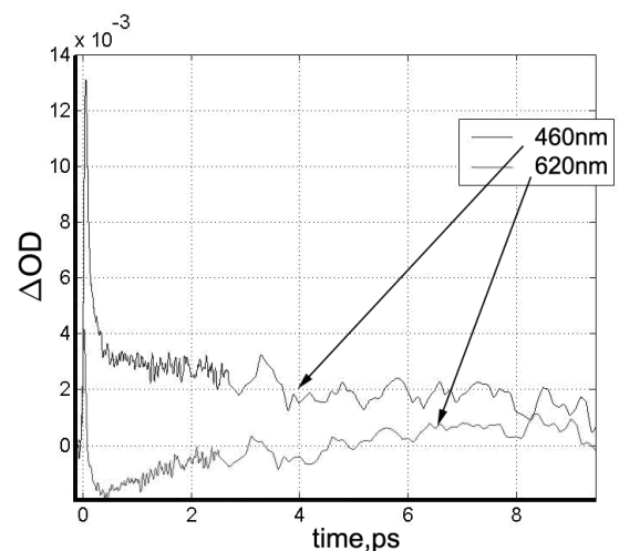
Fig. (7) Au/ \text{TiO}_2 mesoporous film relaxation in pump-probe experiment of femtosecond spectroscopy
