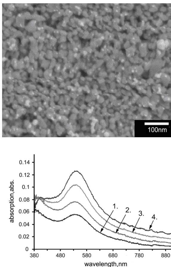
Fig. (2) (a) SEM image of the Me/TiO 2 mesoporous film, (b) experimental absorption spectra of the mesoporous films with various times of nanoparticle deposition: (1) 4 min (2) 8 min (3) 15 min (4) 25 min
