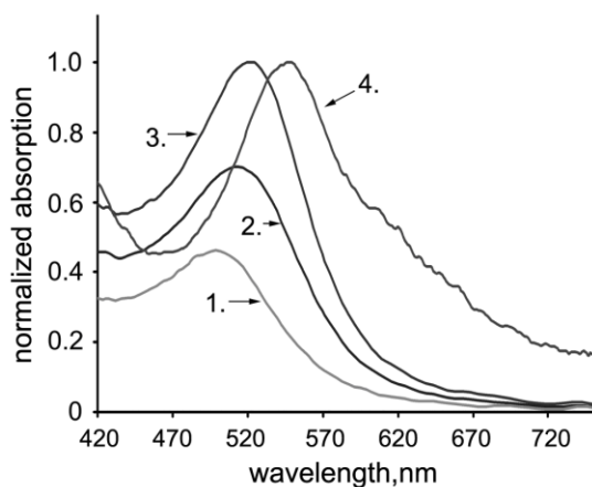
Fig. (5) Absorption spectra (FDTD result) of Au sphere dimer (radius 10nm, distance 2nm) with various polarization of incident light: (1) s-polarization (2) 45° between dimer axis and E (3) p-polarization (4) Au dimer on \text{TiO}_2 surface
