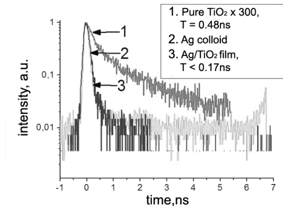
Fig. (6) Kinetic curves of luminescence of pure \text{TiO}_2 , Ag colloid and Ag/ \text{TiO}_2 mesoporous film
