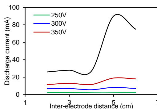
Figure (4) Variation of discharge current with inter-electrode distance at certain discharge voltages without using magnetron
