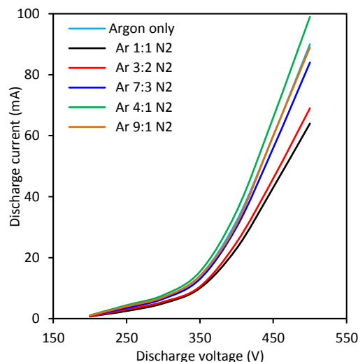
Figure (7) Discharge current-voltage characteristics for different argon/nitrogen mixtures at total gas pressure of 0.7mbar and inter-electrode distance of 4cm
