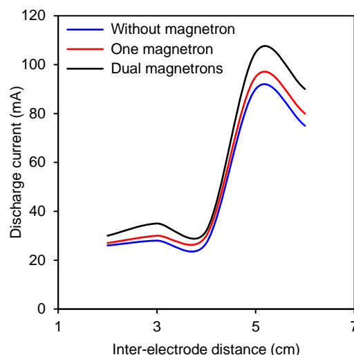
Figure (6) Variation of discharge current with inter-electrode distance at certain discharge voltage (400V) for the cases without magnetron, using one magnetron and dual magnetrons
