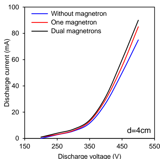
Figure (5) Current-voltage characteristics of discharge plasma at inter-electrode distance of 4cm without magnetron, with only one magnetron and with dual magnetrons
